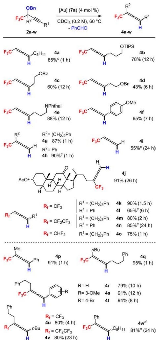
Scheme 2. Substrate Scope: Gold-Catalyzed Formation of Trifluoromethyl-allenes c
