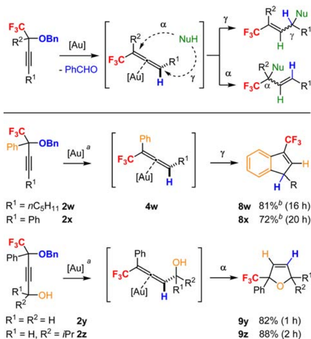
Scheme 3. Gold-Catalyzed Cascade Reactions Involving Trifluoromethyl-allenes Intermediates
