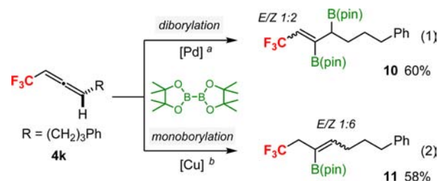
Scheme 4. Copper- and Palladium-Catalyzed Borylation of Trifluoromethyl-allenes
